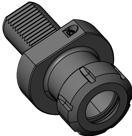
STRAIGHT VDI40 STATIC TOOL OUTPUT: ER40 COOLANT: INTERNAL
